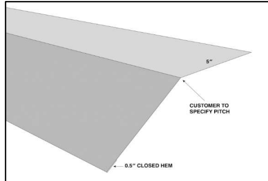
UPPER GAMBREL
