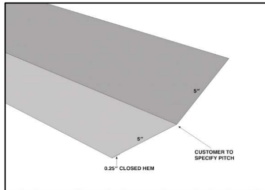
LOWER GAMBREL
