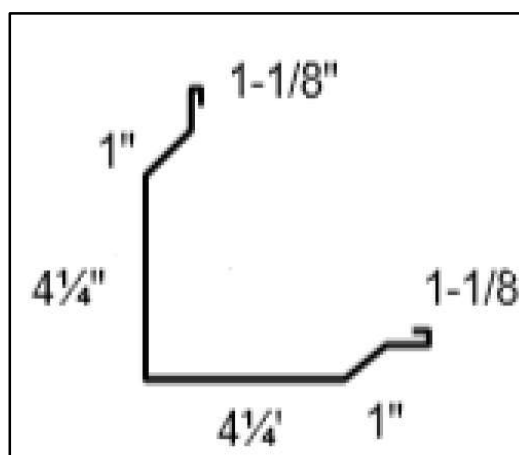
LARGE CORNER
