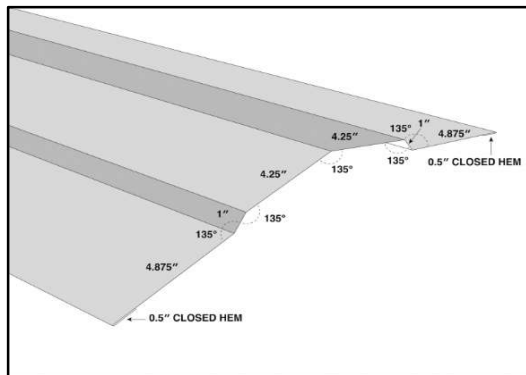
WIDE RIDGECAP
