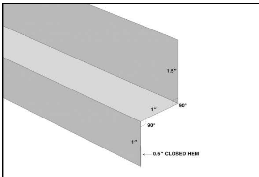
DOUBLE ANGLE
