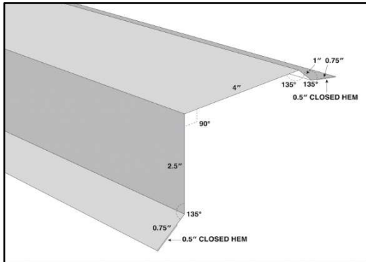
RESIDENTIAL RAKE
