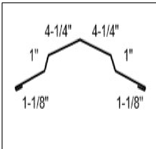
BARN RIDGE
