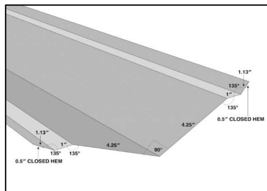
INSIDE CORNER
