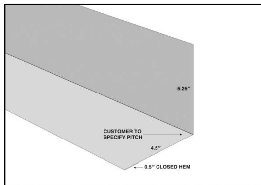
END WALL
