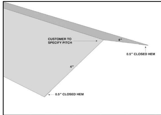
RESIDENTIAL HIP CAP
