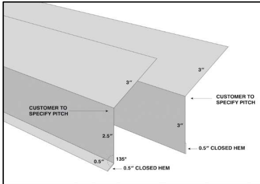
RESIDENTIAL EAVE
