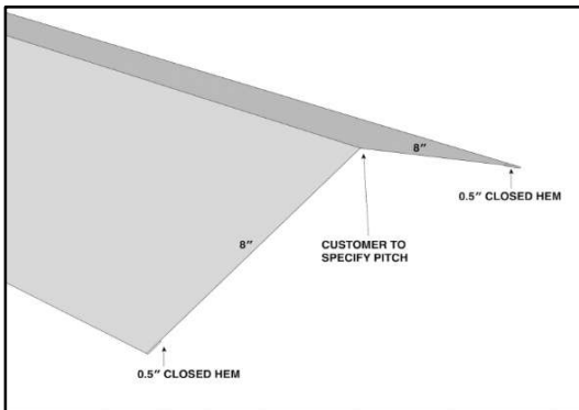
RESIDENTIAL RIDGE CAP
