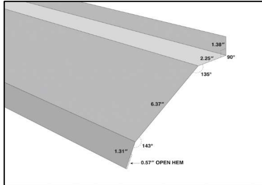
ROUND TRACK COVER
