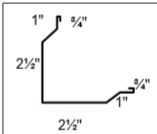
SMALL CORNER
