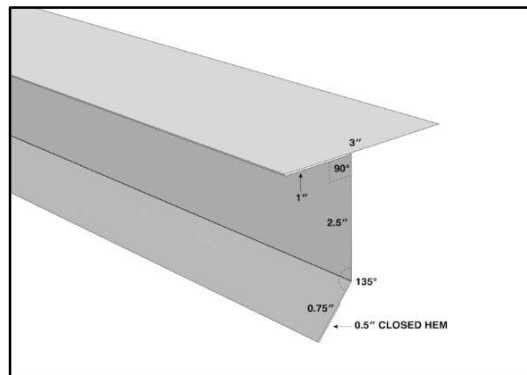
RESIDENTIAL DRIP EDGE
