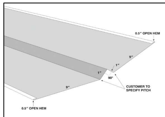
RESIDENTIAL VALLEY
