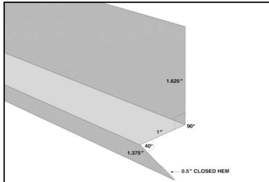
RAT GUARD
