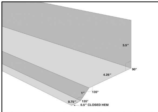
SIDE WALL
