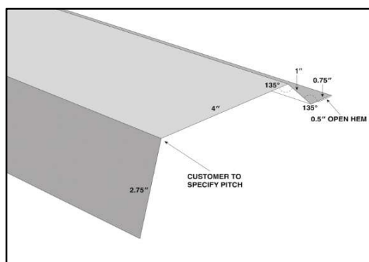
FASCIA
