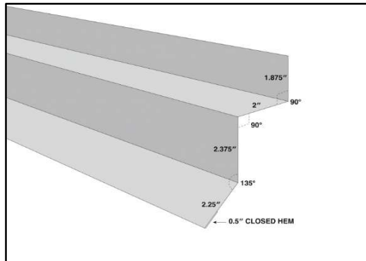
SQUARE TRACK COVER NARROW
