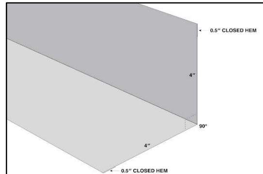
INSIDE ANGLE 4x4
