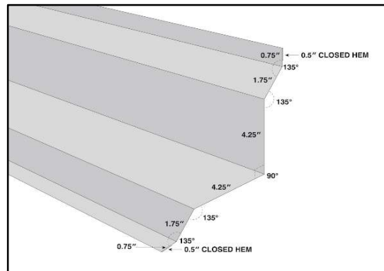
INSIDE CORNER
