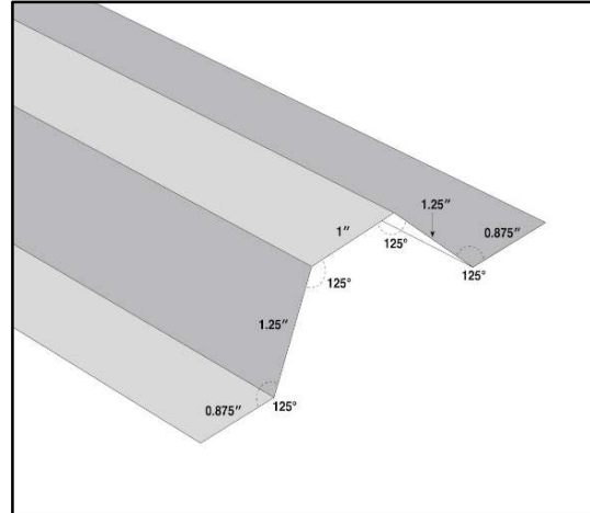
SKYLIGHT TRIM
