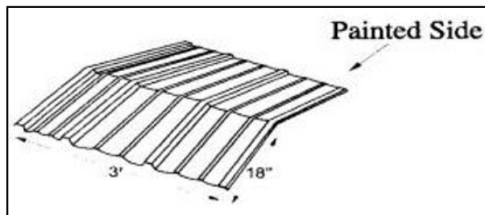
FORMED RIDGE CAP
