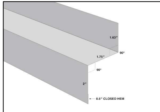
DOUBLE ANGLE
