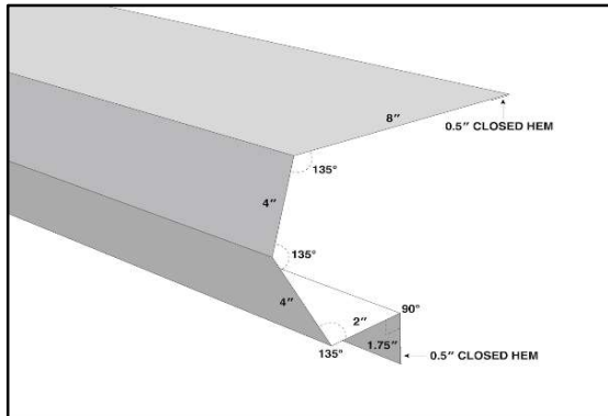
HI-SIDE EAVE
