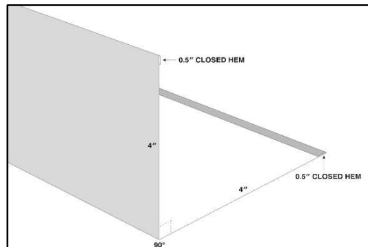
OUTSIDE ANGLE 4x4
