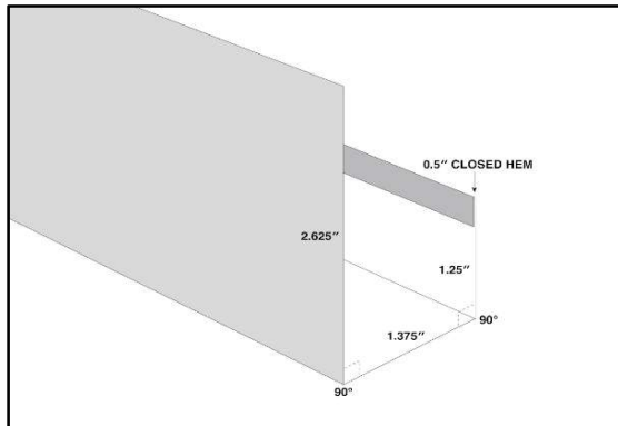
J-TRIM
