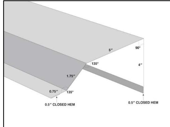
HOUSE RAKE
