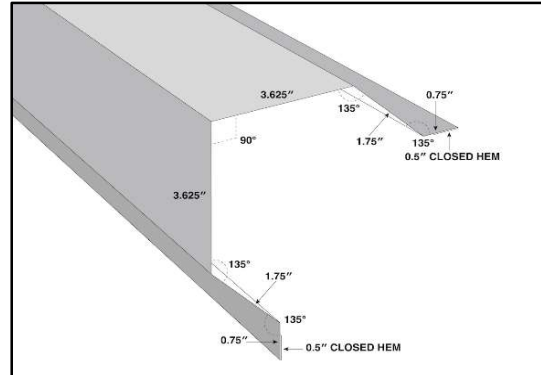
OUTSIDE CORNER
