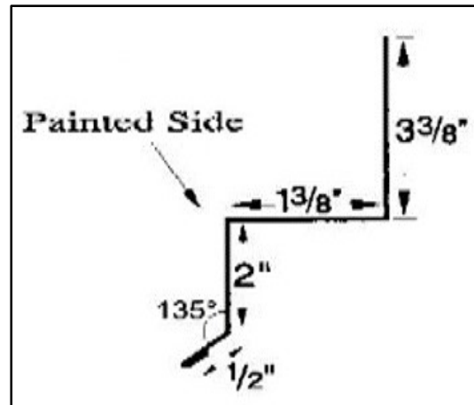
WINDOW CAP
