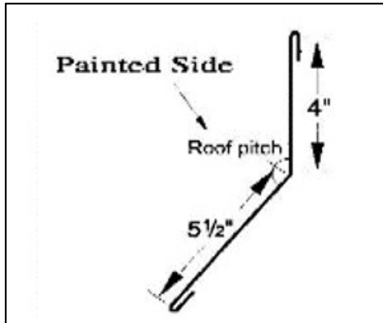
HIGH SIDE PARPET
