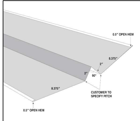
VALLEY
