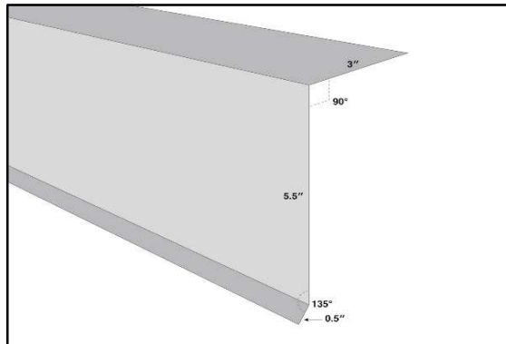
LONG EAVE TRIM
