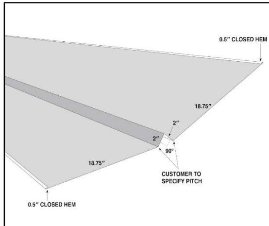
WIDE VALLEY
