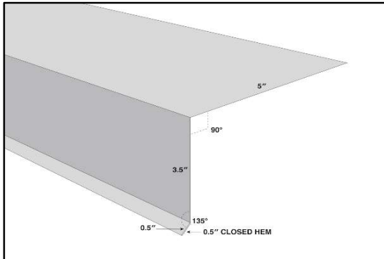
SHORT EAVE
