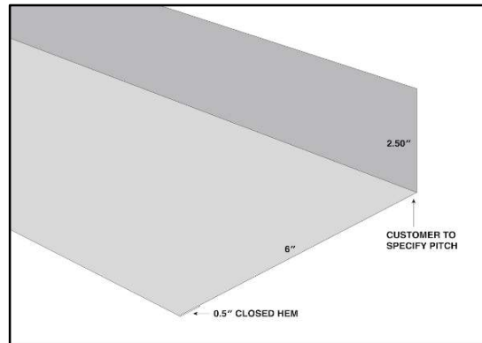
END WALL
