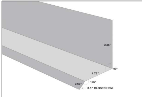
BASE TRIM
