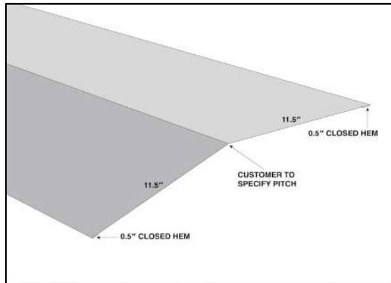
UNIVERSAL RIDGE
